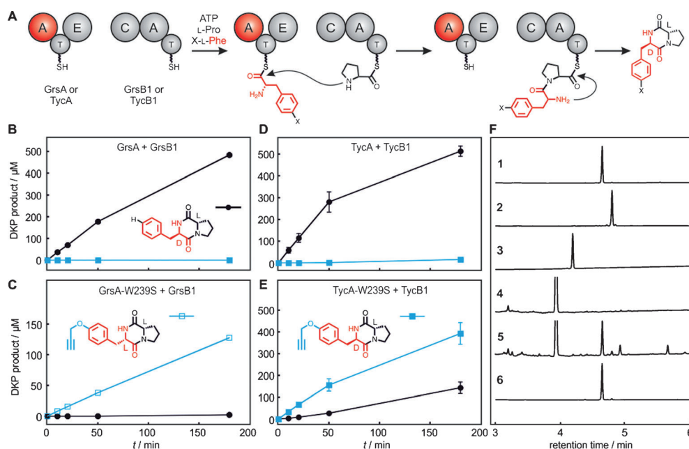
Figure 3. Nonribosomal synthesis of propargylated DKP. A) Mechanism of nonribosomal DKP formation by the truncated NRPSS. B–E) Kinetics of DKP formation from 500 \mu\text{M} L-Pro, L-Phe, and O -propargyl-L-Tyr as competing substrates were determined with different dimodular synthetases: B) GrsA/GrsB1, C) GrsA-W239S/GrsB1, D) TycA/TycB1, and E) TycA-W239S/TycB1. k_{\text{obs}} values are summarized in Table S2. Concentrations of D-Phe-L-Pro DKP (black circles), O -propargyl-L-Tyr-L-Pro DKP (open cyan squares), and O -propargyl-D-Tyr-L-Pro DKP (cyan squares) were determined by UPLC. F) UPLC traces of DKP standards (1: O -propargyl-D-Tyr-L-Pro DKP, 2: O -propargyl-L-Tyr-L-Pro DKP, 3: D-Phe-L-Pro DKP) and propargyl DKP produced in vivo (4: reaction t = 0 h, 5: t = 24 h, 6: purified product). The peak at 3.9 minutes corresponds to O -propargyl-L-Tyr. Traces were normalized to the height of the DKP peak.
